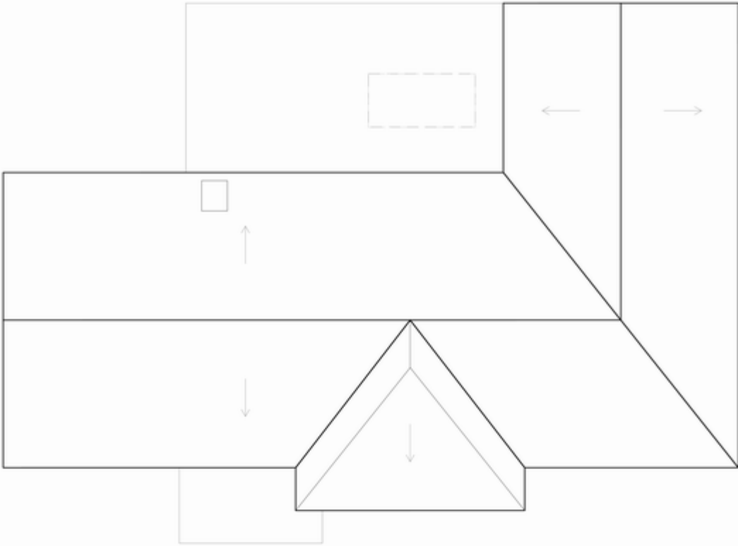
3 Proposed Roof Plan Scale: 1:100
